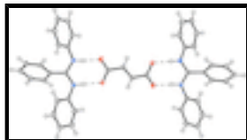
Fig. 2. Crystal structure of the title compound with view of the trimers (hydrogen bonding is indicated by dashed lines).
